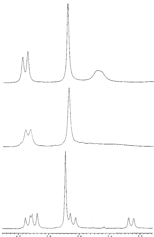
Figure 4. 400 MHz ^1\text{H} NMR spectra of the methylene protons of 7 (in \text{CDCl}_3 ) at different temperatures. From bottom to top: at 230 K, 282 K, and 310 K.
