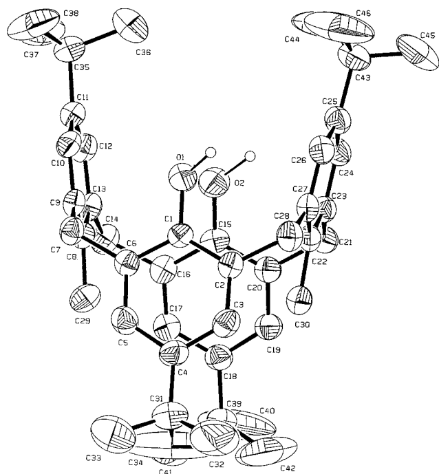
Figure 2. Crystal structure of tetra- tert -butyl-25,27-dihydroxy-26,28-dimethylcalix[4]arene ( 6 ). The large thermal ellipsoids of the methyls of the tert -Bu groups are due to rotational disorder of the groups.
